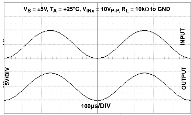
FIGURE 26. OPERATION WITH RAIL-TO-RAIL INPUT AND
